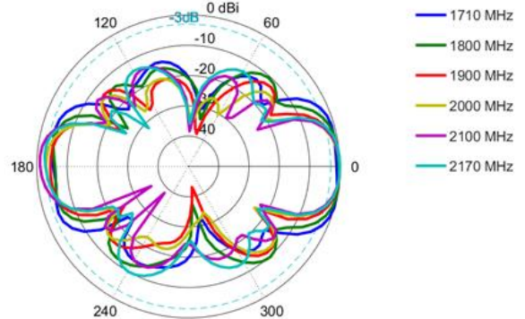
Elevation: 1710 – 2170 MHz
